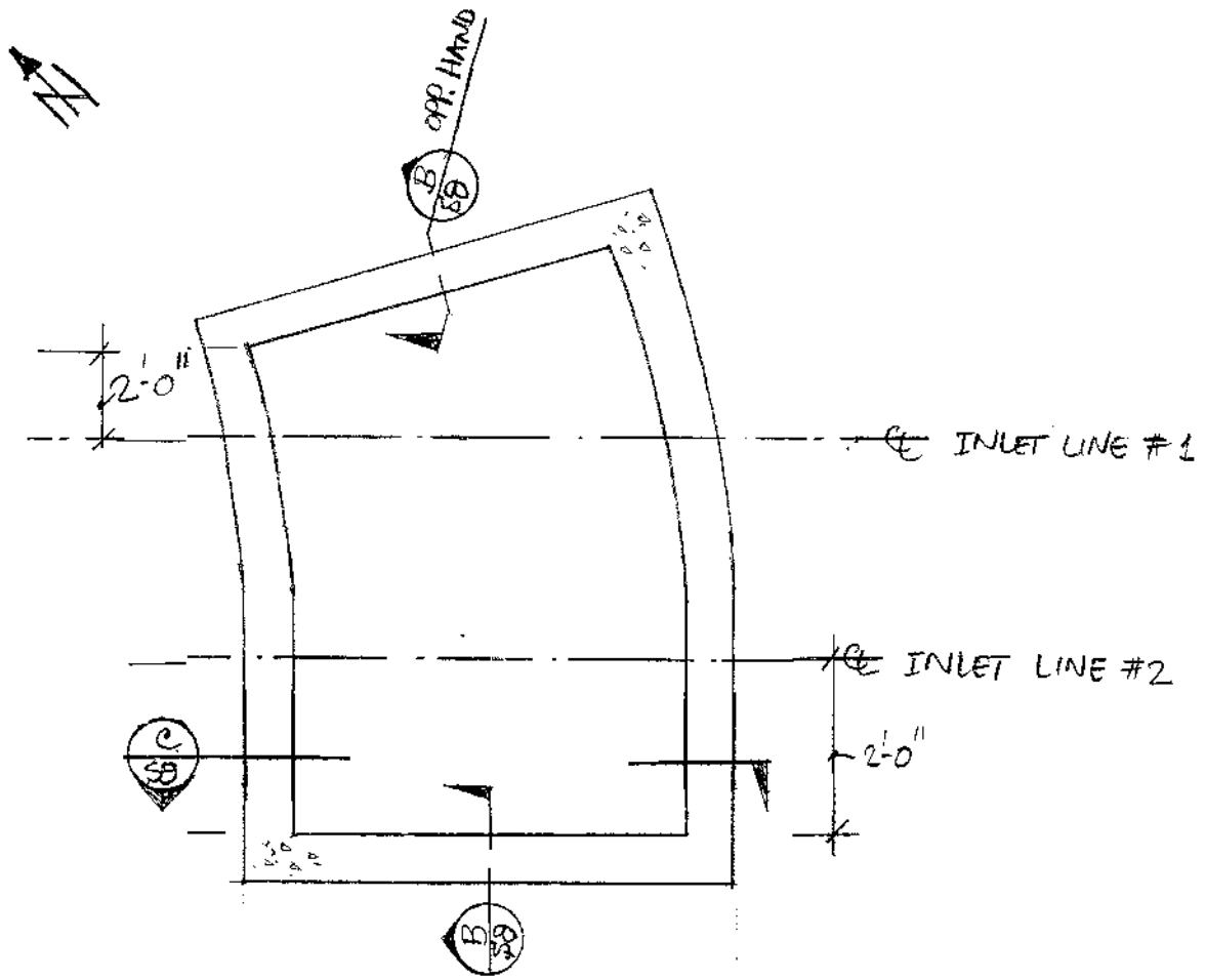
PLAN VAULT FOR INLET PIPELINE & VALVE
