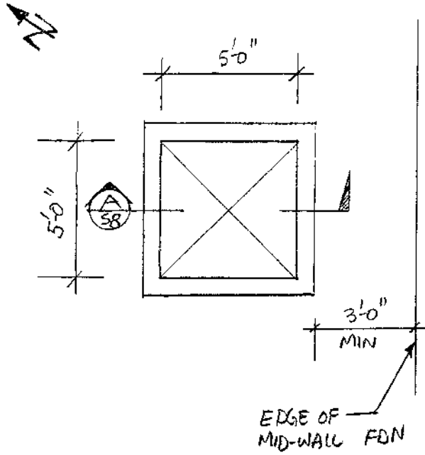
SUMP DETAIL (1/58)
