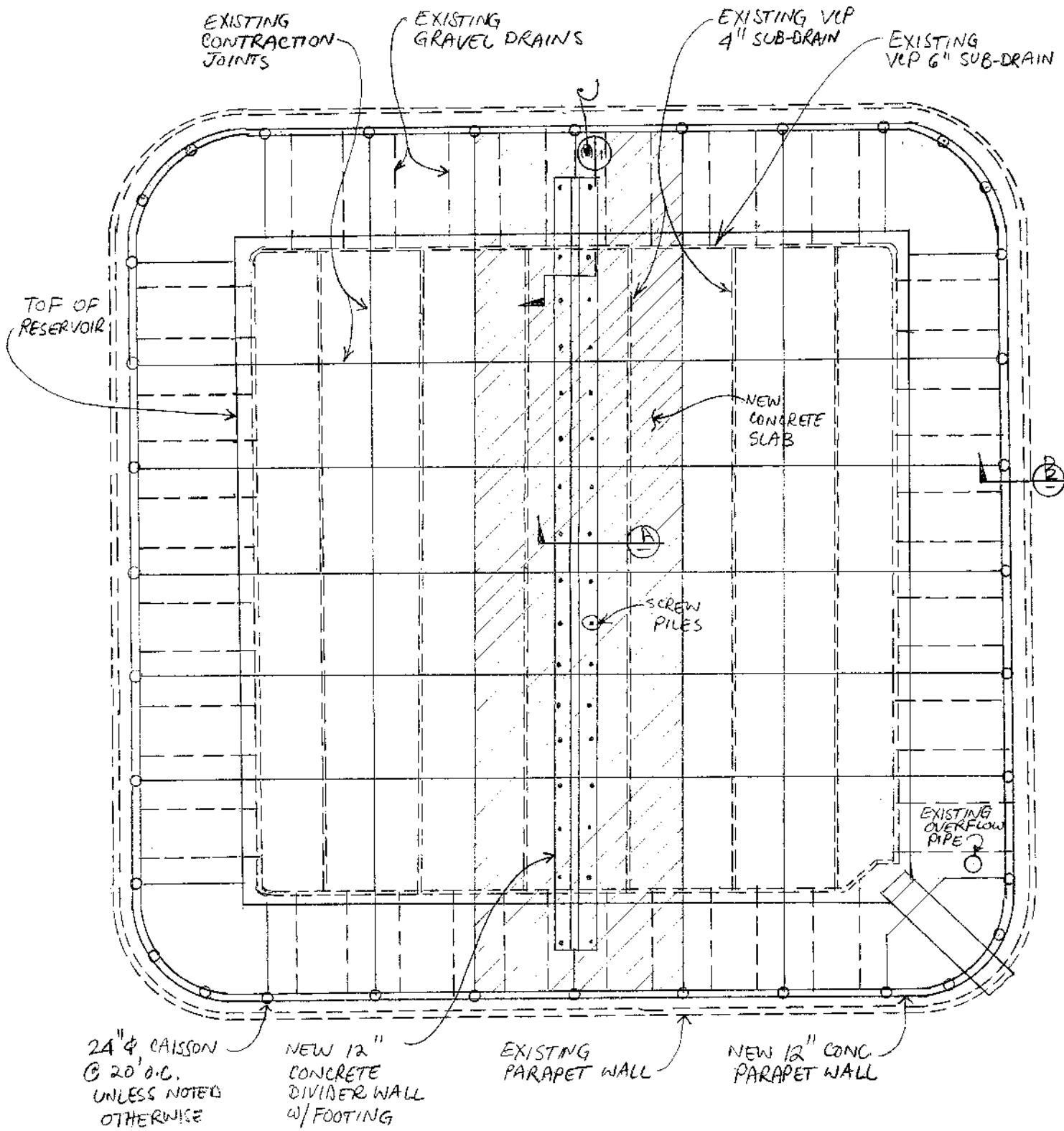
PLAN DIVIDER WALL, PARAPET WALL & FOUNDATIONS
